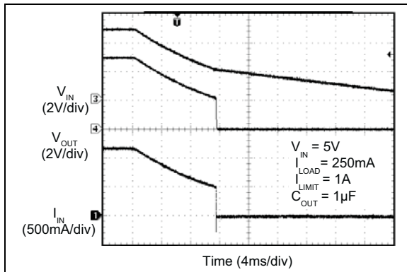
FIGURE 2-14: Soft-Start Turn-Off.
