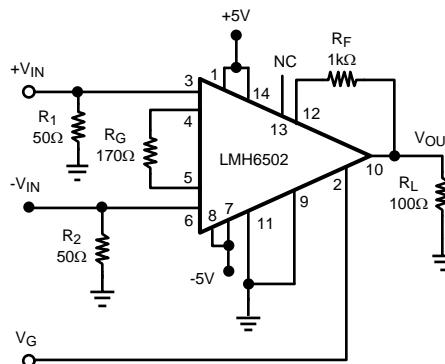
Figure 2. A_{VMAX} = 10V/V
