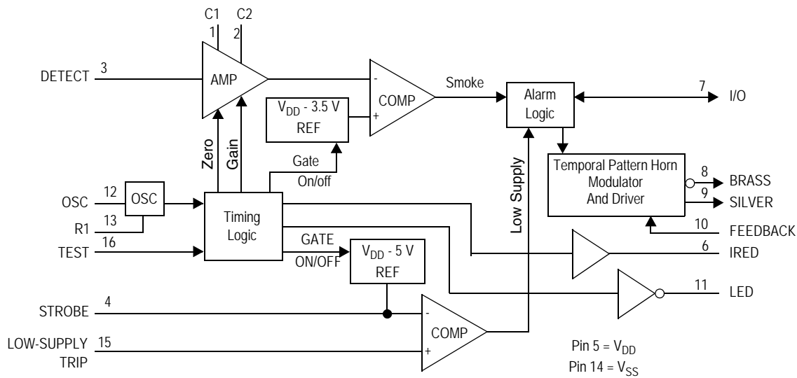
Figure 2. Block Diagram
