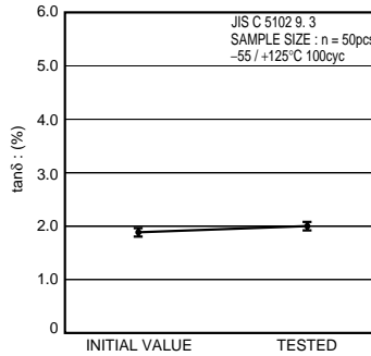
Fig.11 tanδ
