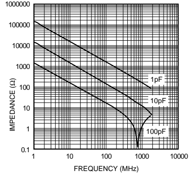
Fig.2 Impedance-frequency characteristics
