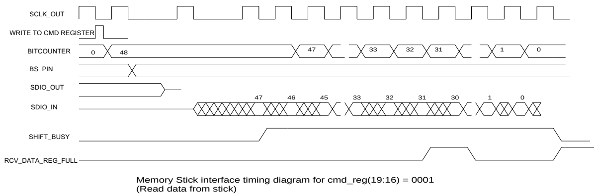
Figure 13-11 Reading Data From MemoryStick Timing
