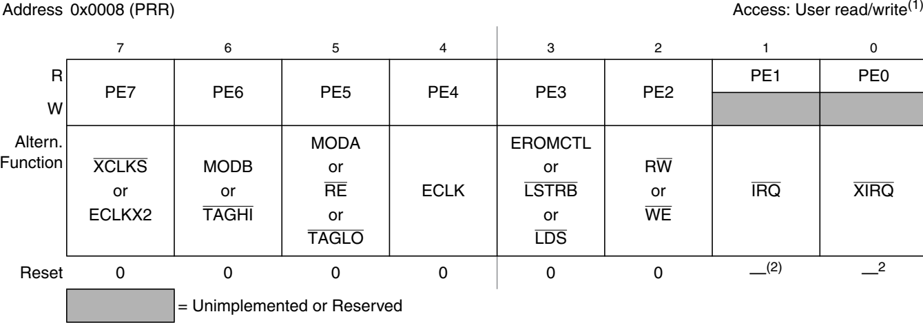
Figure 2-9. Port E Data Register (PORTE)
