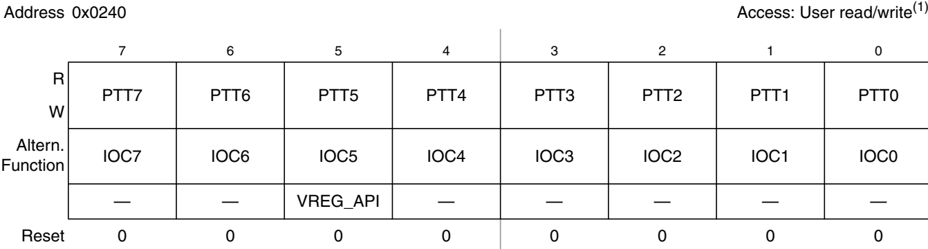
Figure 2-19. Port T Data Register (PTT)
