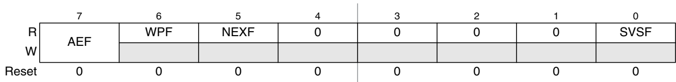
Figure 4-3. MPU Flag Register (MPUFLG)
