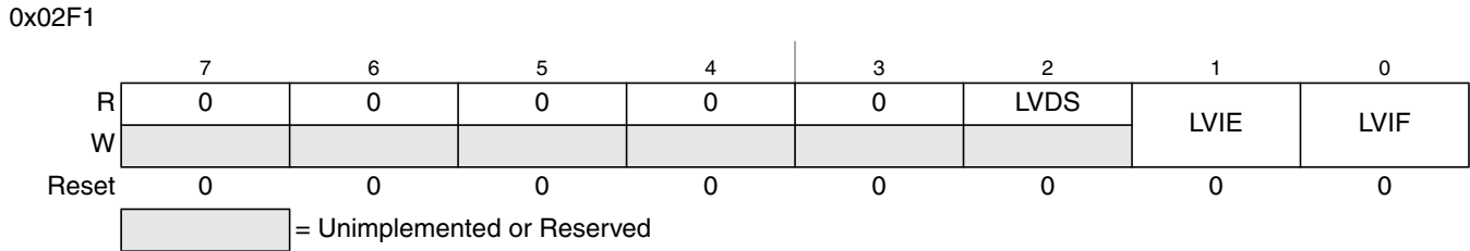
Figure 23-3. Control Register (VREGCTRL)
