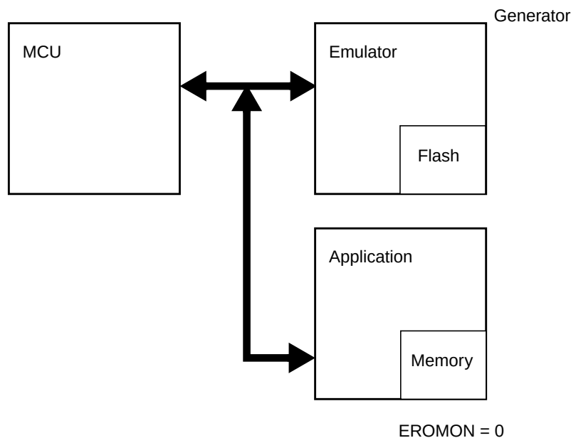
Figure 17-30. ROMON = 1 in Emulation Expanded Mode
