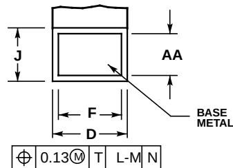
SECTION J1-J1
