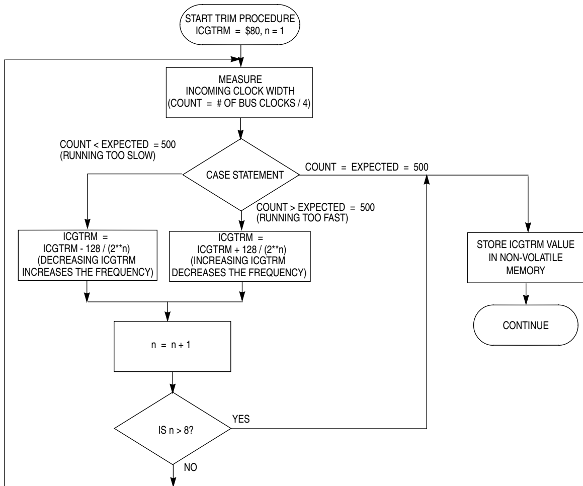
Figure 9-17. Trim Procedure
