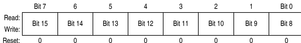
Figure 16-4. Break Address Register High (BRKH)
