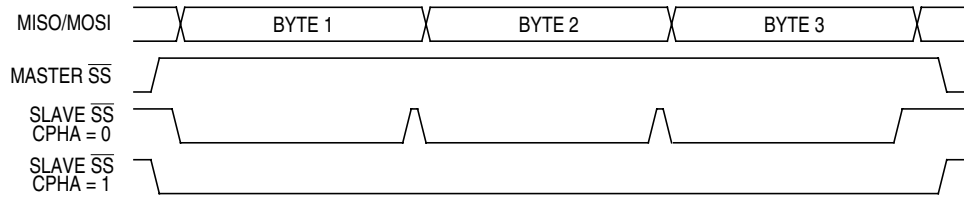
Figure 15-12. CPHA/SS Timing
