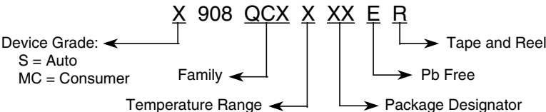
Figure 20-1. Device Numbering System
