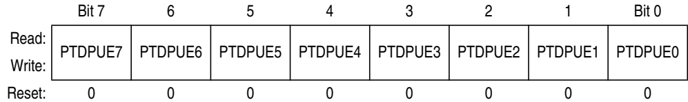
Figure 11-16. Port D Input Pullup Enable Register (PTDPUE)
