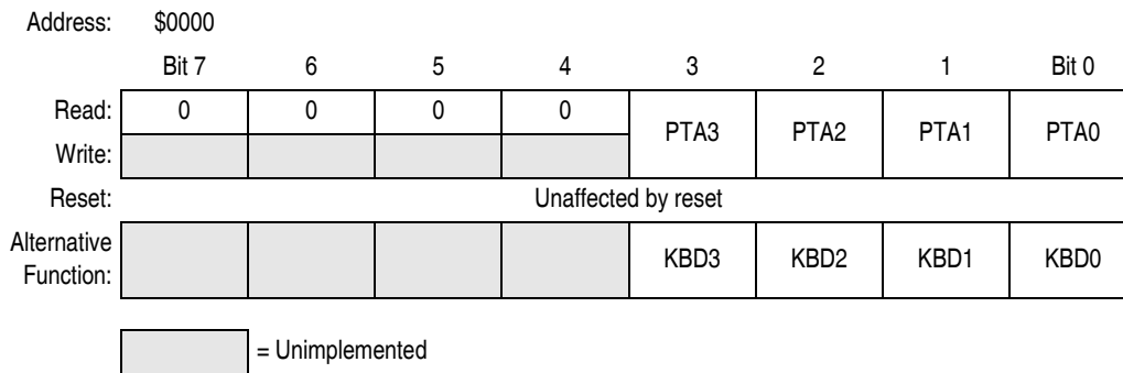
Figure 12-2. Port A Data Register (PTA)
