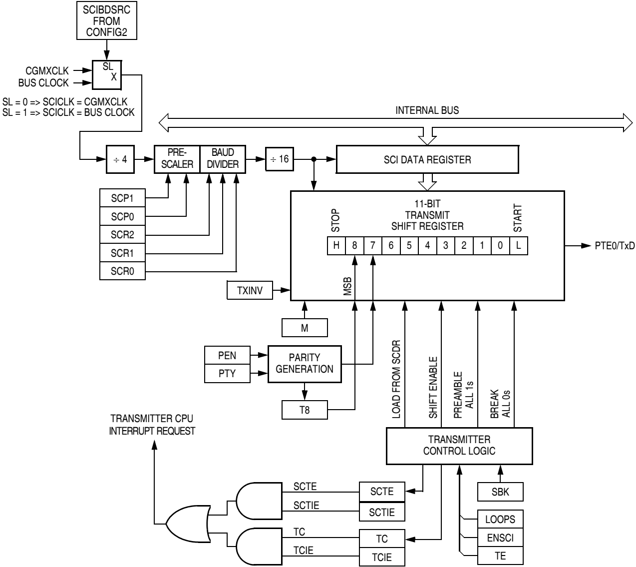
Figure 13-5. SCI Transmitter
