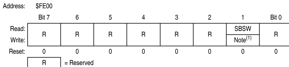
Figure 14-20. Break Status Register (SBSR)
