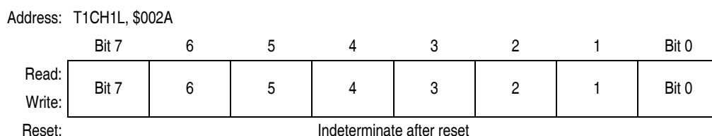
Figure 17-16. TIM Channel 1 Register Low (TCH1L)
