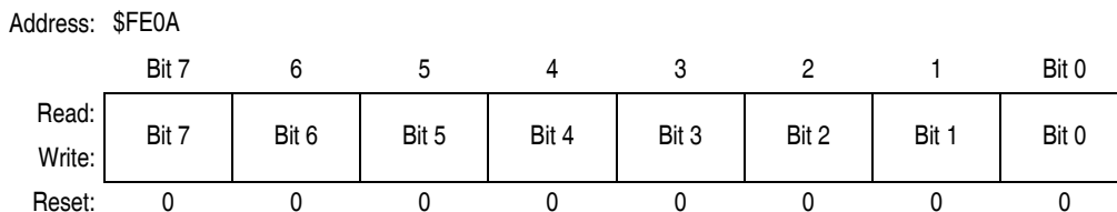
Figure 18-6. Break Address Register Low (BRKL)
