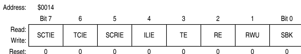
Figure 13-11. SCI Control Register 2 (SCC2)
