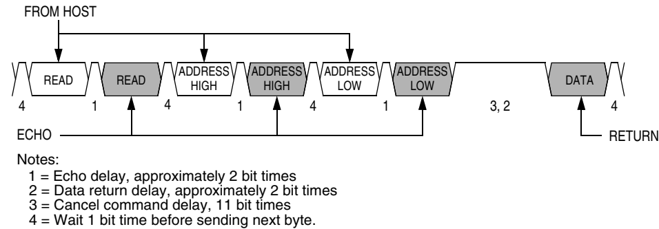
Figure 19-14. Read Transaction
