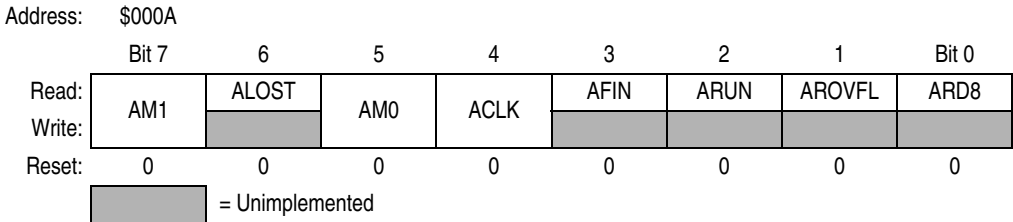
Figure 14-19. ESCI Arbiter Control Register (SCIACTL)
