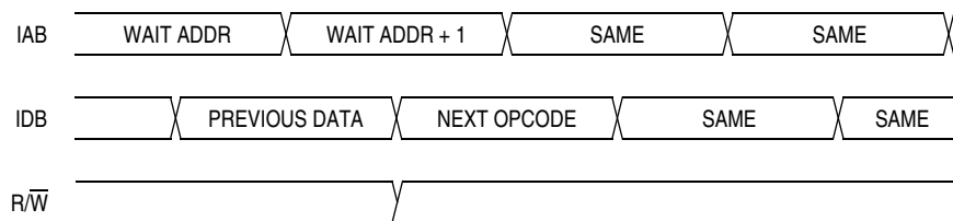
Figure 15-15. Wait Mode Entry Timing
