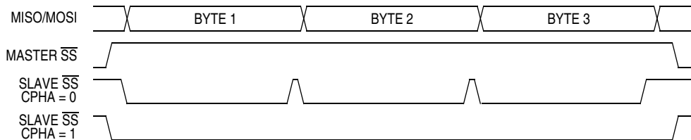
Figure 16-6. CPHA/\overline{SS} Timing
