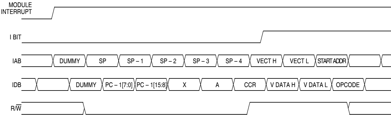
Figure 14-7. Interrupt Entry
