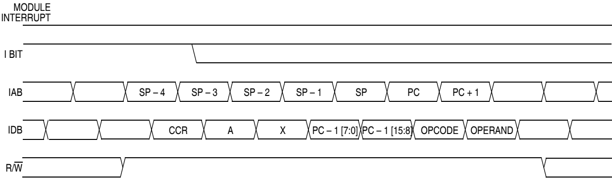
Figure 14-8. Interrupt Recovery
