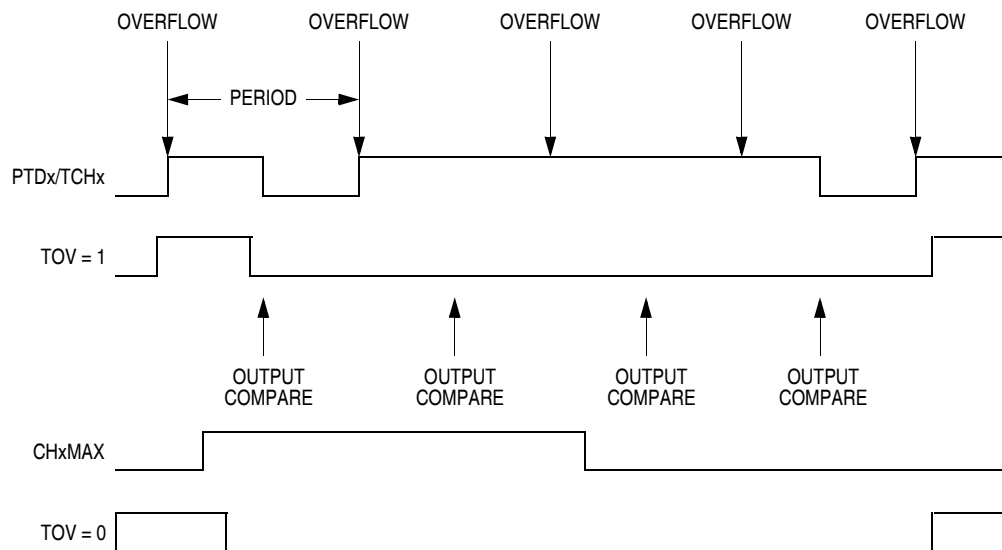
Figure 17-8. CHxMAX Latency
