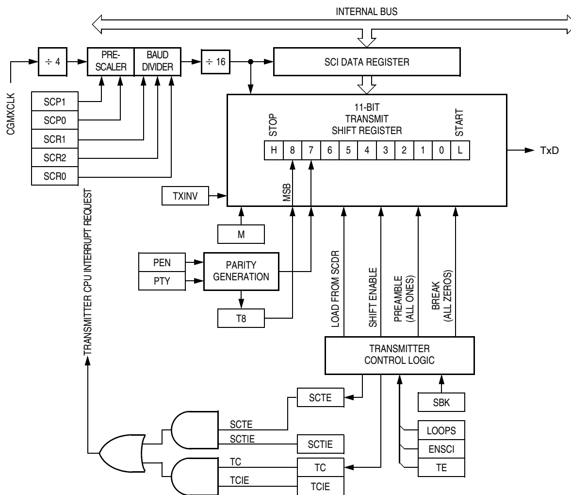
Figure 16-4. SCI Transmitter
