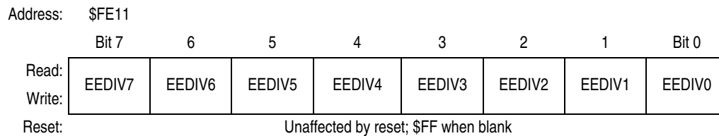
Figure 5-8. EEPROM Divider Nonvolatile Register Low (EEDIVLNVR)
