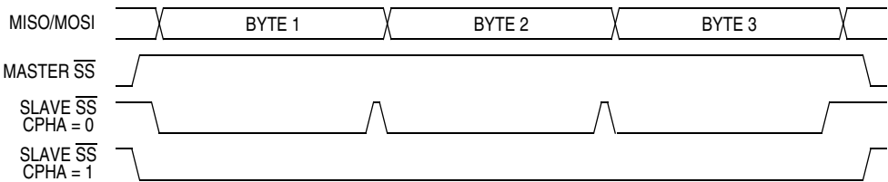
Figure 17-11. CPHA/ \overline{SS} Timing
