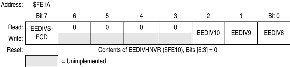
Figure 5-5. EEDIV Divider High Register (EEDIVH)
