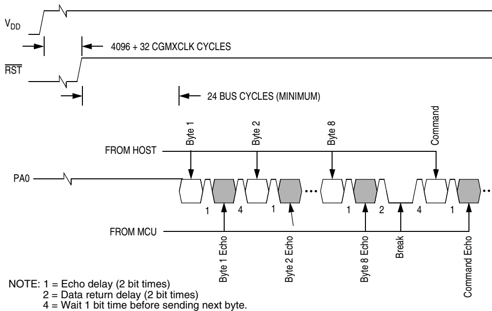
Figure 12-6. Monitor Mode Entry Timing
