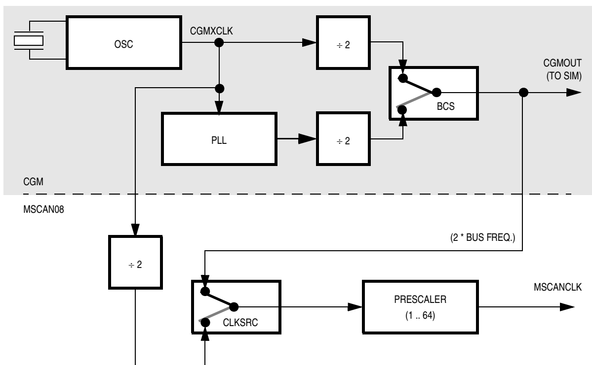
Figure 24-7. Clocking Scheme
