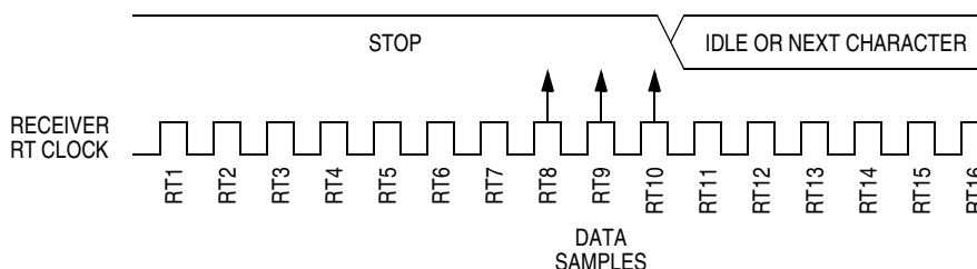
Figure 16-10. Fast Data
