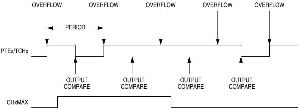
Figure 19-8. CHxMAX Latency
