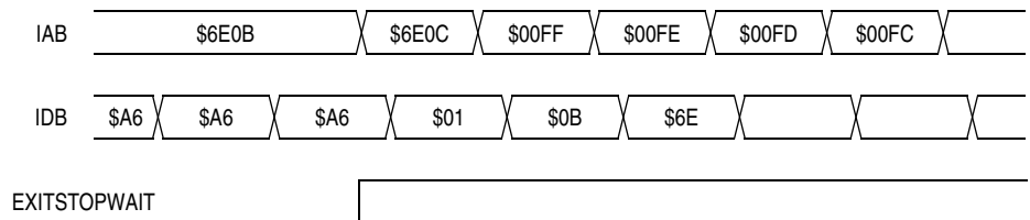
Figure 7-12. Wait Mode Entry Timing
