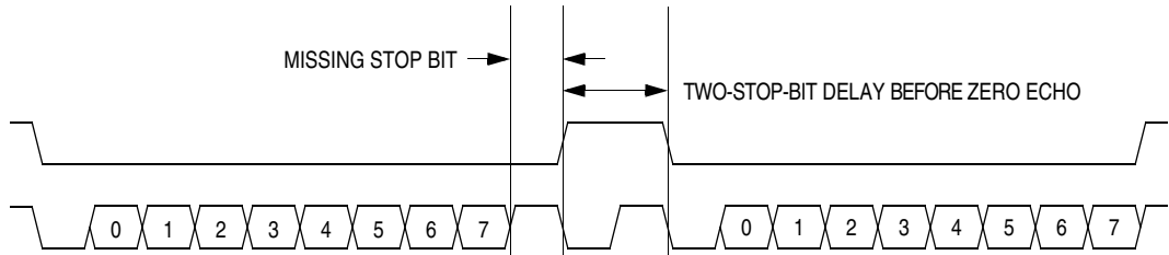
Figure 12-5. Break Transaction
