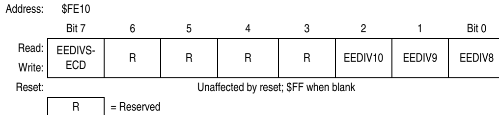
Figure 5-7. EEPROM Divider Nonvolatile Register High (EEDIVHNVR)
