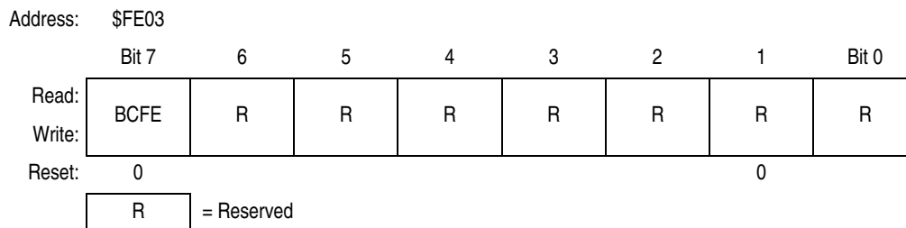
Figure 7-19. SIM Break Flag Control Register (SBFCR)
