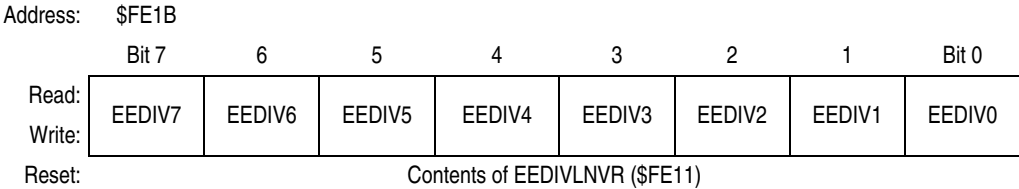
Figure 5-6. EEDIV Divider Low Register (EEDIVL)
