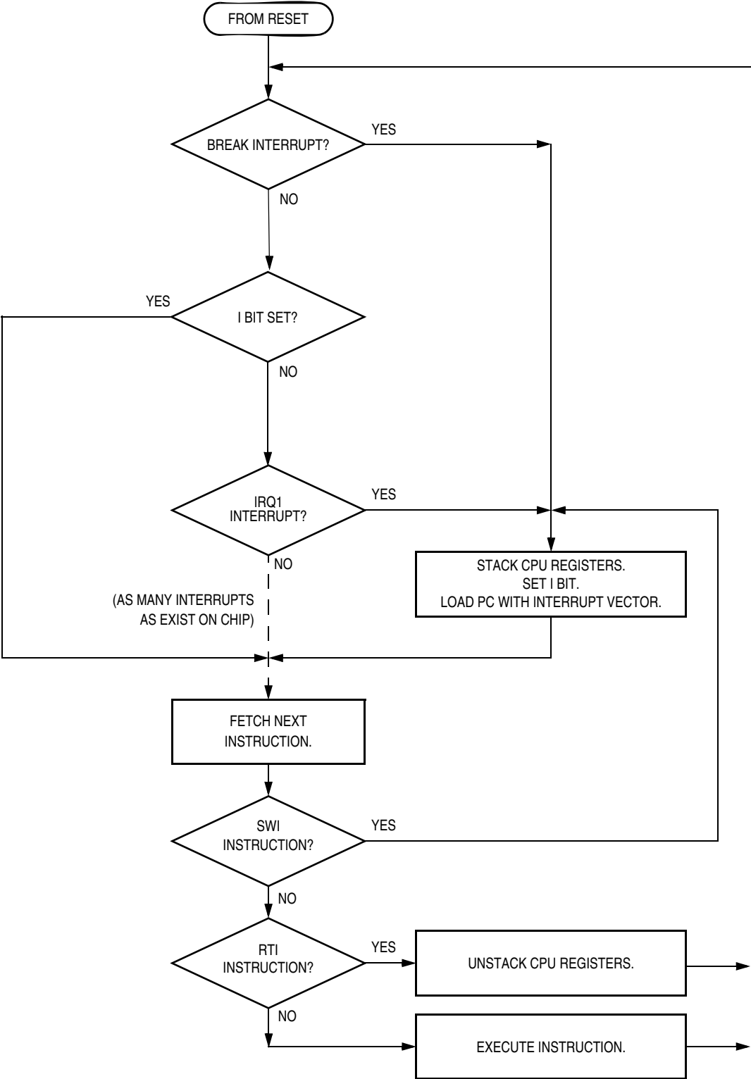
Figure 7-10. Interrupt Processing
