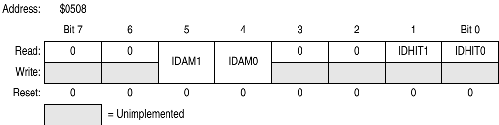
Figure 24-23. Identifier Acceptance Control Register (CIDAC)
