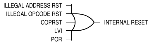
Figure 15-6. Sources of Internal Reset
