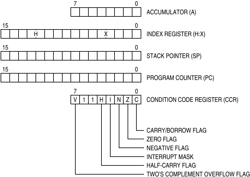
Figure 9-1. CPU Registers
