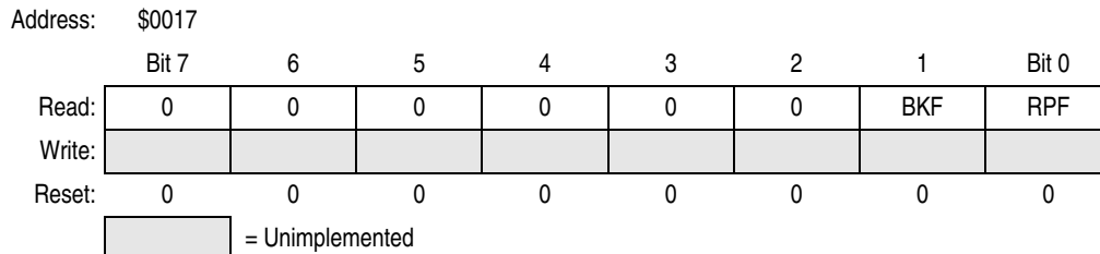
Figure 14-14. SCI Status Register 2 (SCS2)
