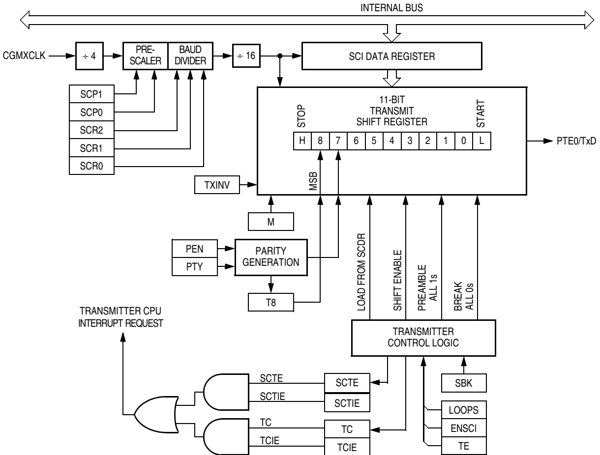
Figure 14-4. SCI Transmitter
