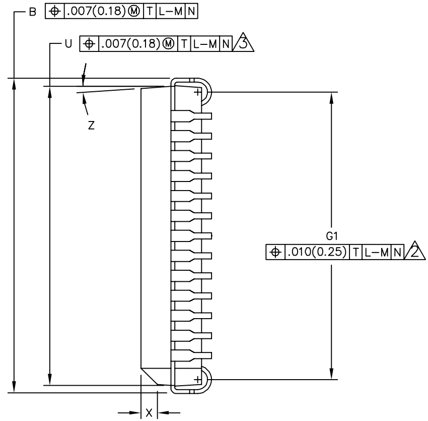
VIEW D-D
