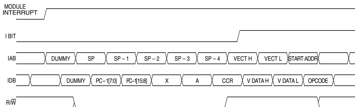
Figure 15-8. Interrupt Entry
