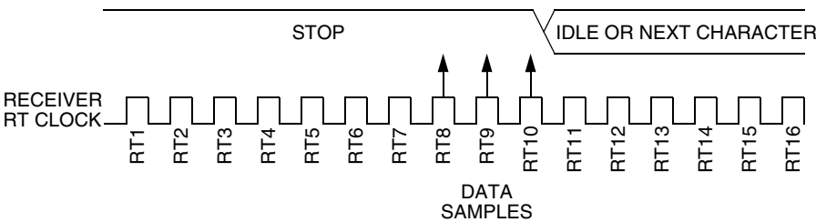
Figure 16-8. Fast Data
