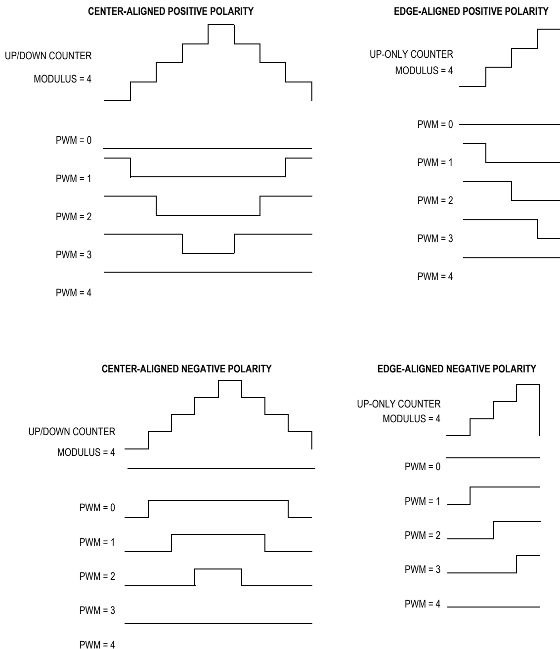
Figure 9-17. PWM Polarity
