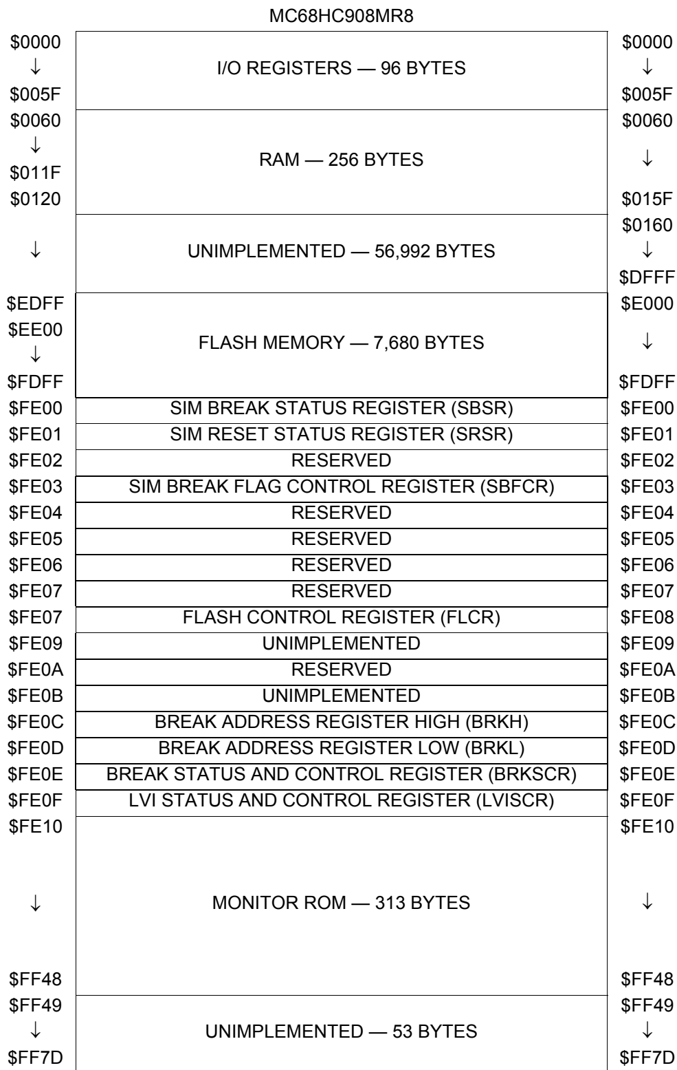
Figure 2-1. Memory Map
