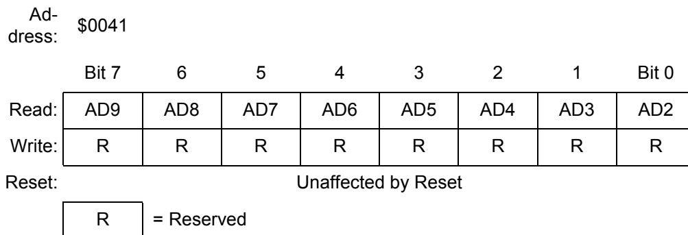
Figure 18-4. ADC Data Register High (ADRH) Left Justified Mode
