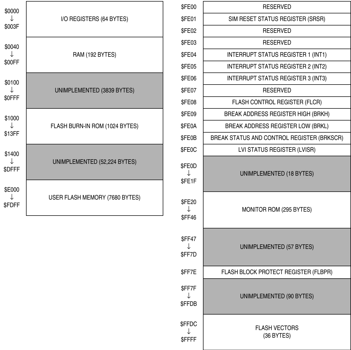
Figure 2-1. Memory Map
