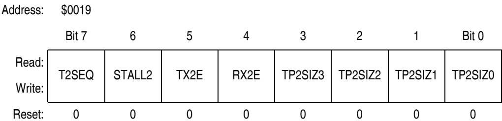
Figure 11-21. USB Control Register 2 (UCR2)
