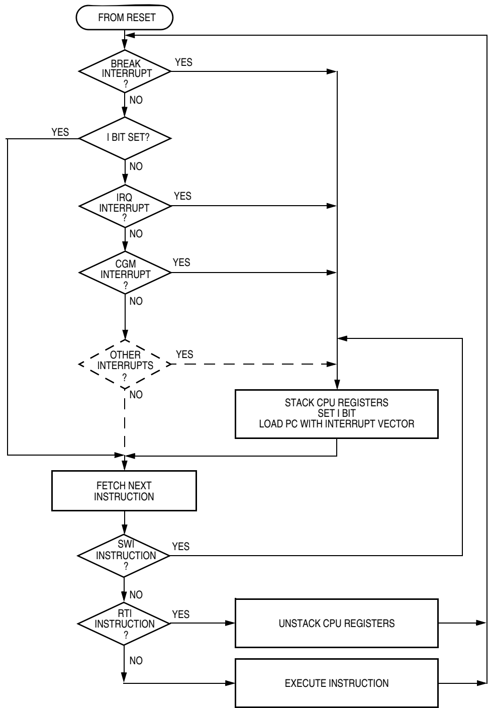
Figure 14-5. Interrupt Processing
