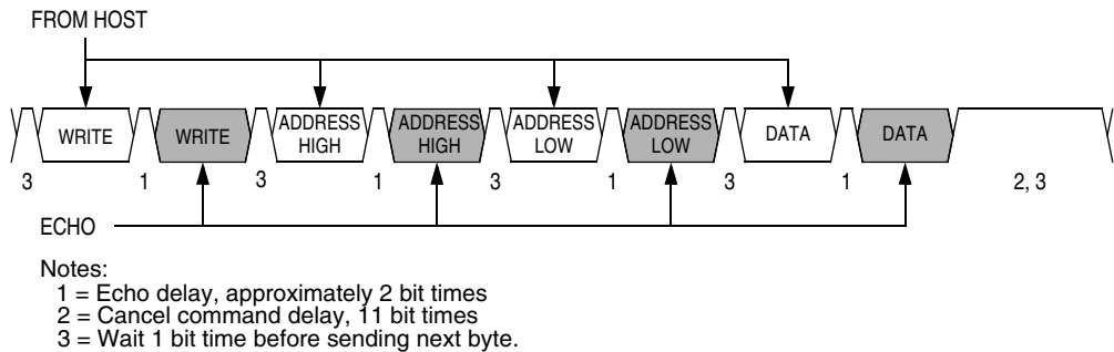
Figure 20-14. Write Transaction
