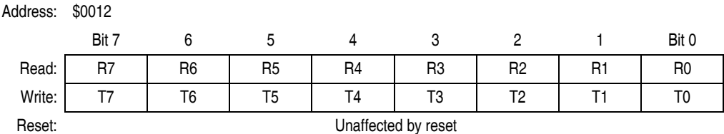
Figure 16-16. SPI Data Register (SPDR)
