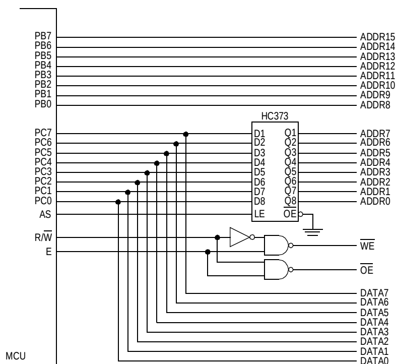
Figure 4-1. Address/Data Demultiplexing
