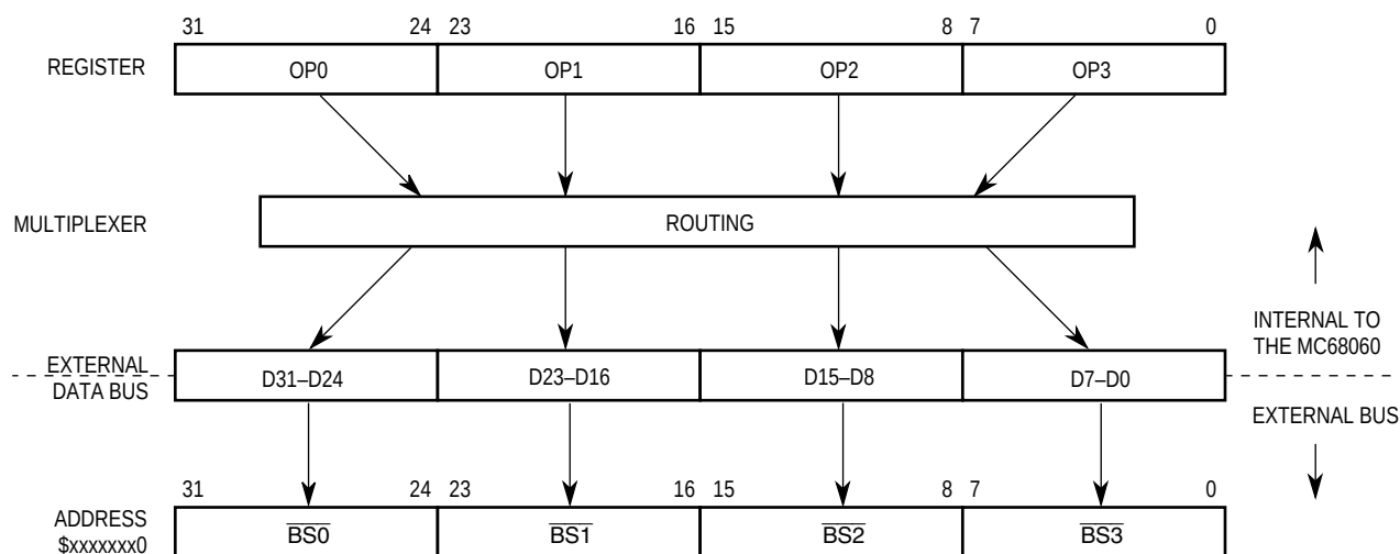
Figure 7-7. Data Multiplexing
