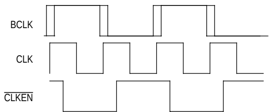
Figure 11-10. MC68040 BCLK to \overline{\text{CLKEN}} Relationship
