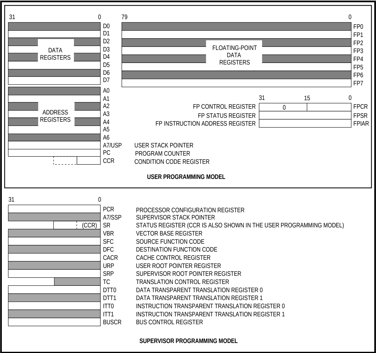
Figure 1-2. Programming Model
