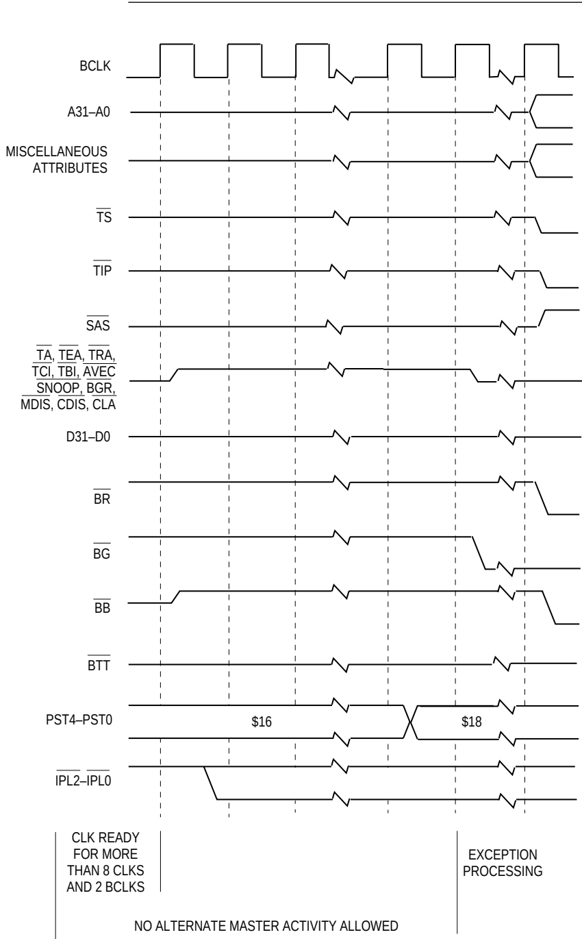
Figure 7-36. Exiting LPSTOP Mode Timing Diagram
