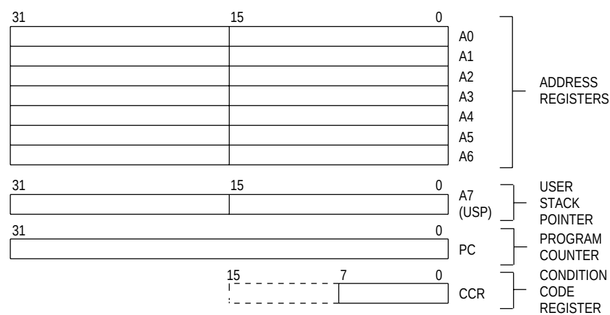
Figure 3-2. Integer Unit User Programming Model
