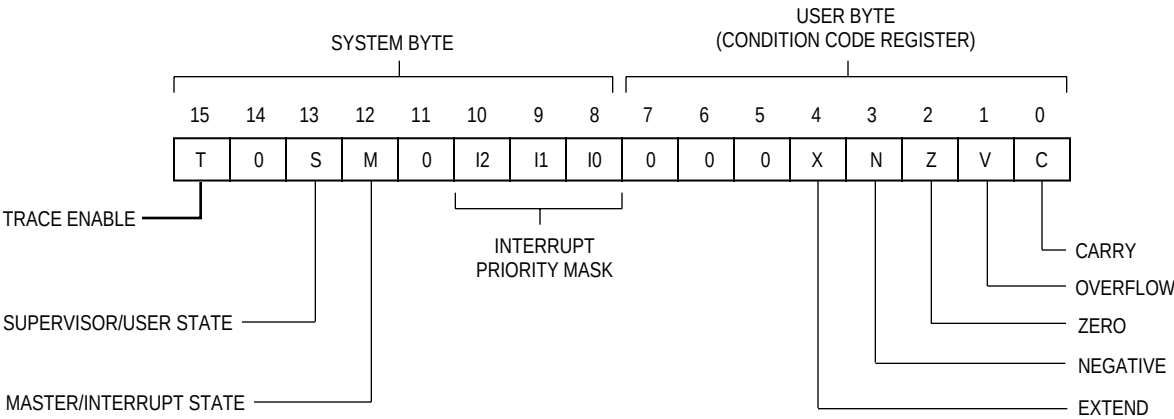
Figure 3-4. Status Register
