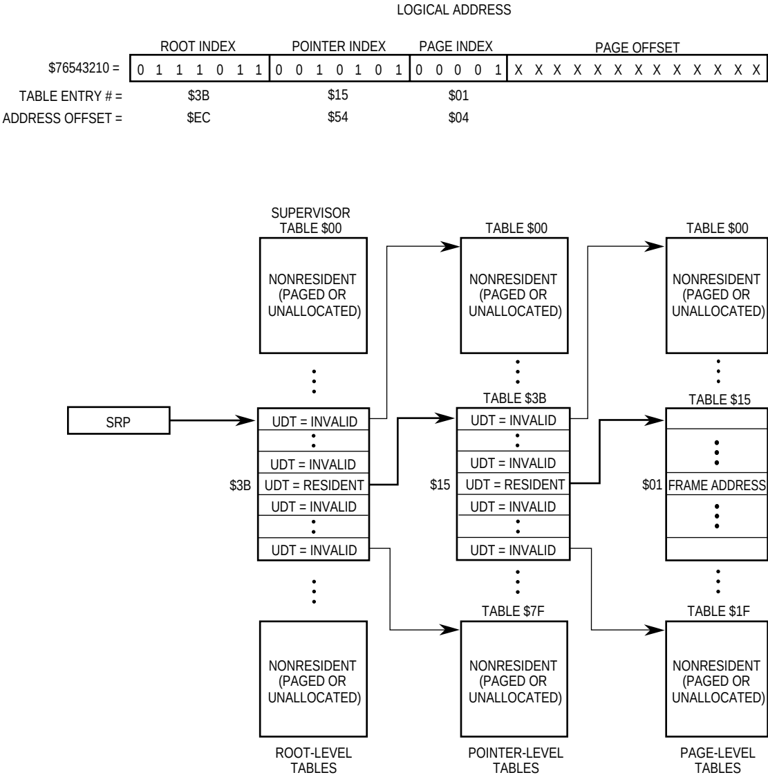
Figure 4-15. Translation Table with Nonresident Tables
