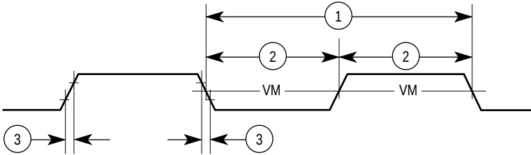
Figure 6-8. Clock Input Timing Diagram
