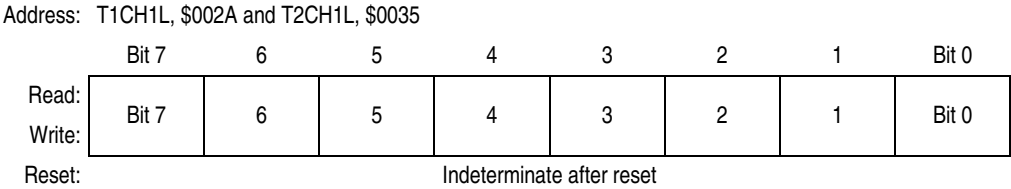
Figure 19-16. TIM Channel 1 Register Low (TCH1L)
