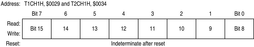
Figure 19-15. TIM Channel 1 Register High (TCH1H)
