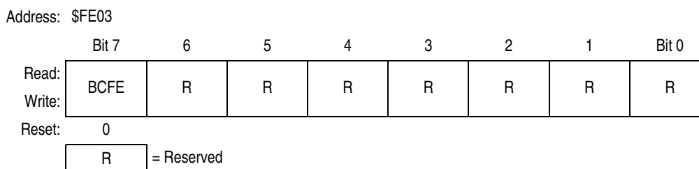
Figure 20-7. Break Flag Control Register (BFCR)
