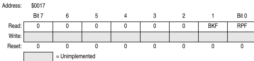
Figure 15-15. ESCI Status Register 2 (SCS2)
