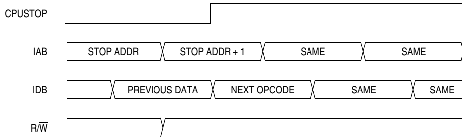
Figure 16-18. Stop Mode Entry Timing
