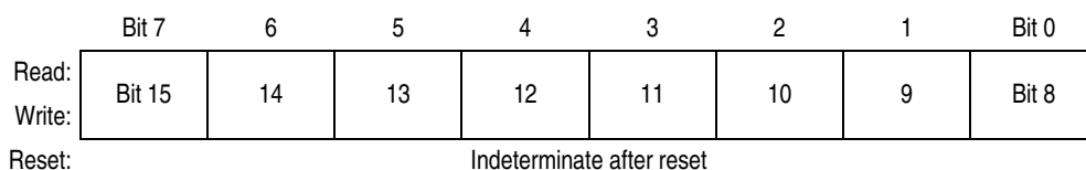
Figure 19-13. TIM Channel 0 Register High (TCH0H)
