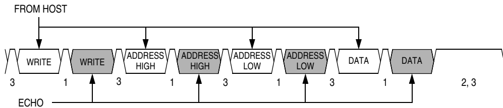
Figure 20-13. Read Transaction
