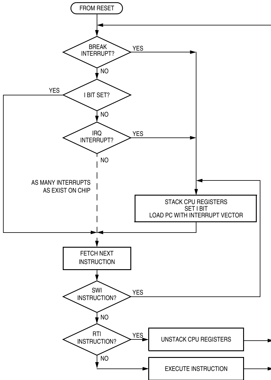
Figure 16-10. Interrupt Processing
