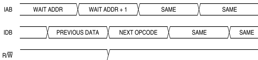
Figure 16-15. Wait Mode Entry Timing
