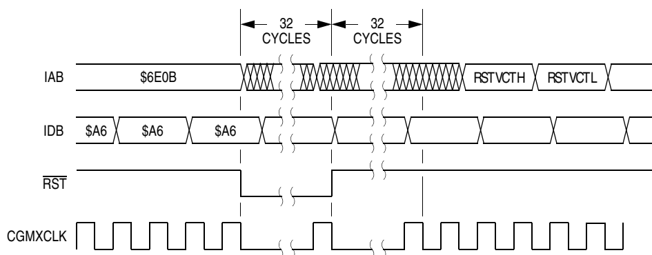
Figure 16-17. Wait Recovery from Internal Reset
