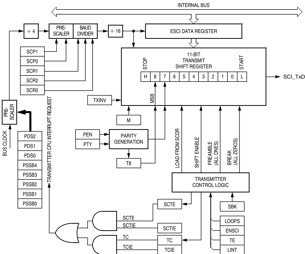
Figure 15-5. ESCI Transmitter
