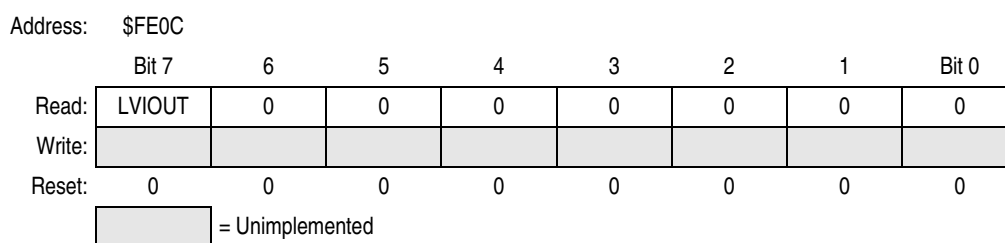
Figure 11-3. LVI Status Register (LVISR)
