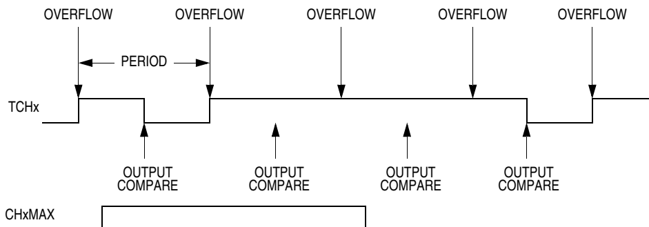
Figure 19-12. CHxMAX Latency
