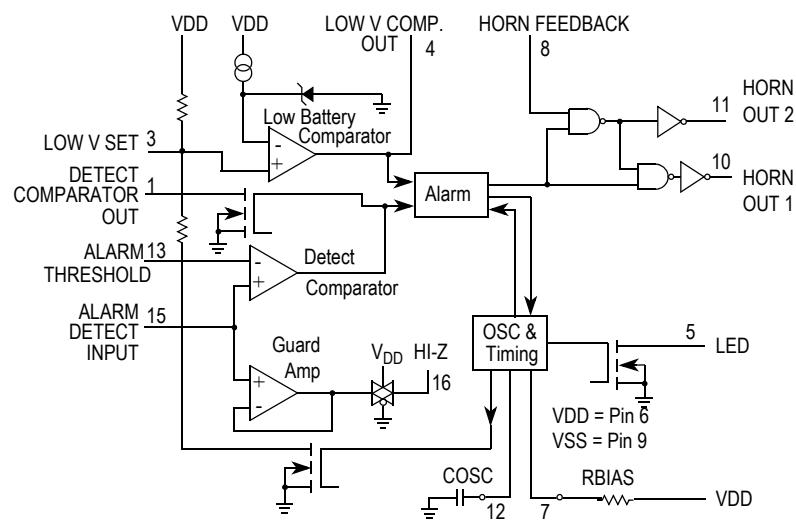
Figure 2. 14600 Block Diagram
