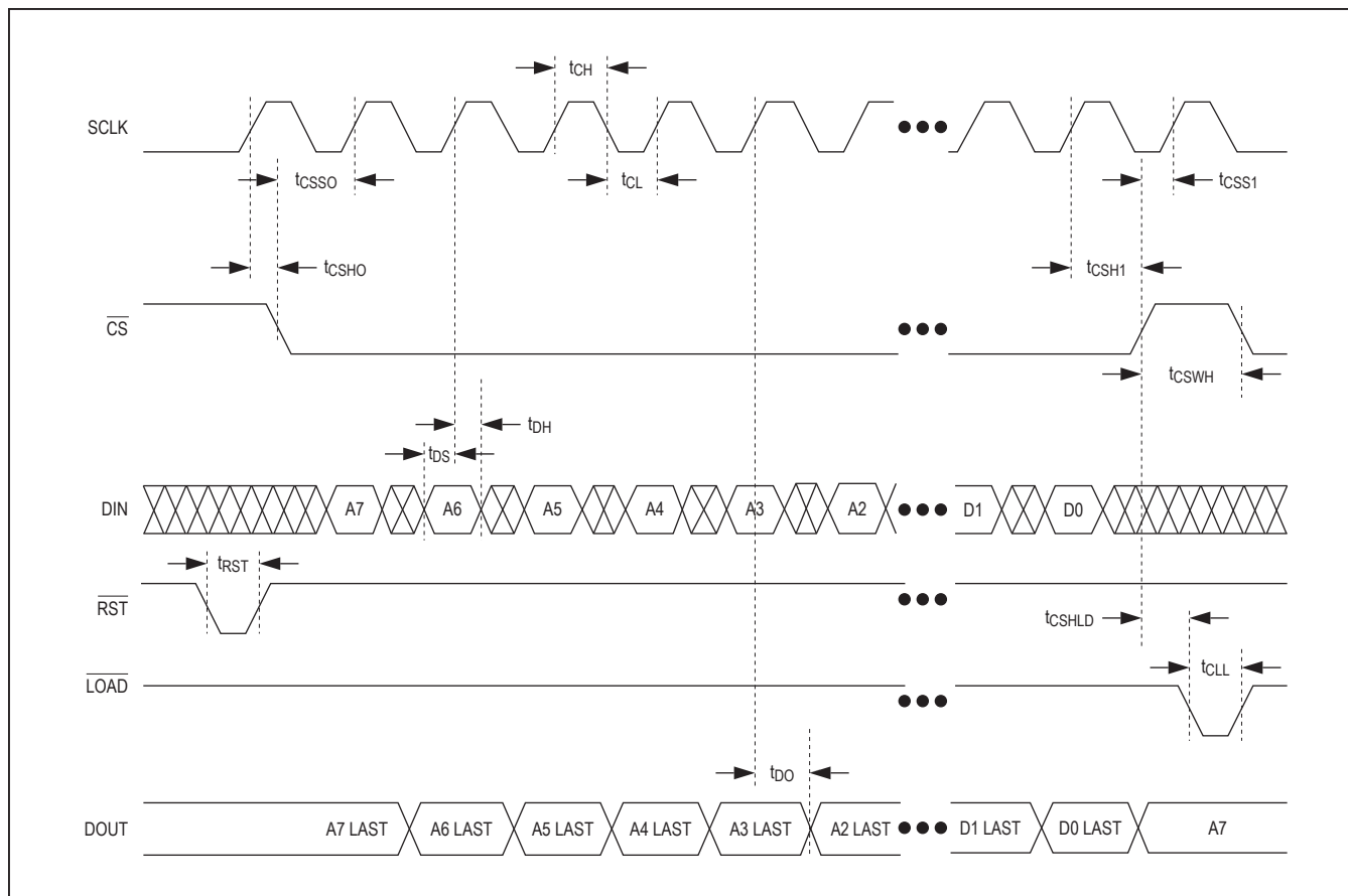
Figure 9. Serial-Interface Timing
