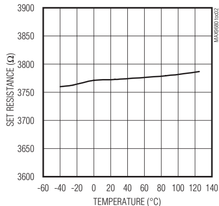
SET RESISTANCE vs. TEMPERATURE
