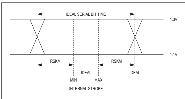
Figure 4. LVDS Receiver Input Skew Margin
