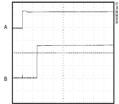
POWER-UP DELAY (OUT)
