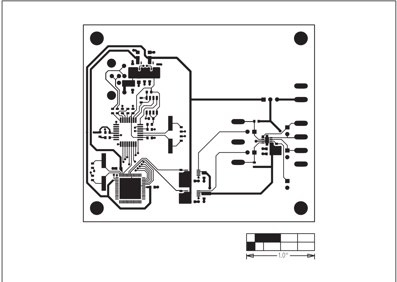
Figure 6. MAX5432 EV Kit PCB Layout—Component Side
