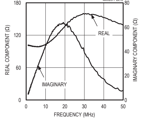
DIFFERENTIAL OUTPUT IMPEDANCE vs. FREQUENCY
