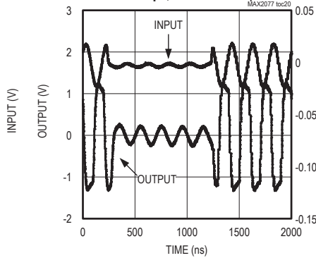
VGA OVERLOAD RECOVERY TIME ( V_{IN} = 40mV_{p-p} FOR 1\mu s TO 4mV_{p-p} FOR 1\mu s AND BACK TO 40mV_{p-p} FOR 1\mu s , GAIN = 42.5dB)
