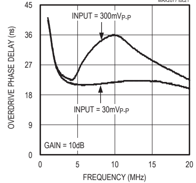
OVERDRIVE PHASE DELAY vs. FREQUENCY
