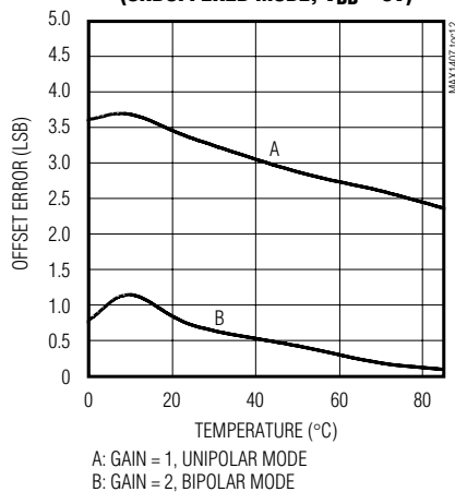
UNCORRECTED OFFSET ERROR vs. TEMPERATURE (UNBUFFERED MODE, V_{DD} = 3V )
