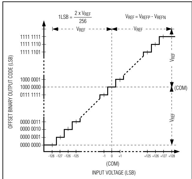
Figure 6. Transfer Function
