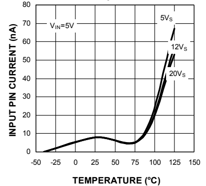
Input Pin Current (IIN) vs. Temperature
