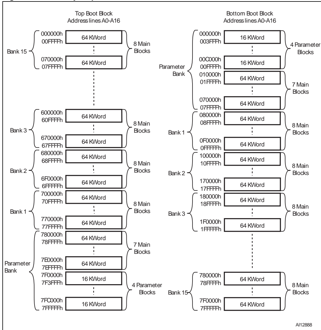
Figure 3. Memory map
