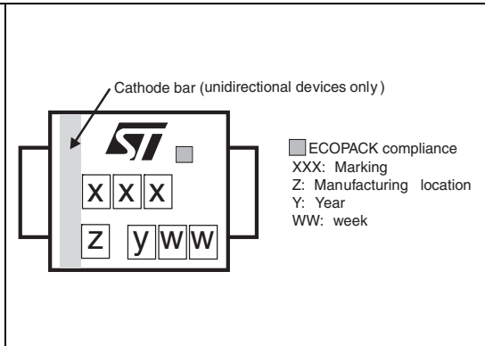
Figure 24. Marking layout (1)
