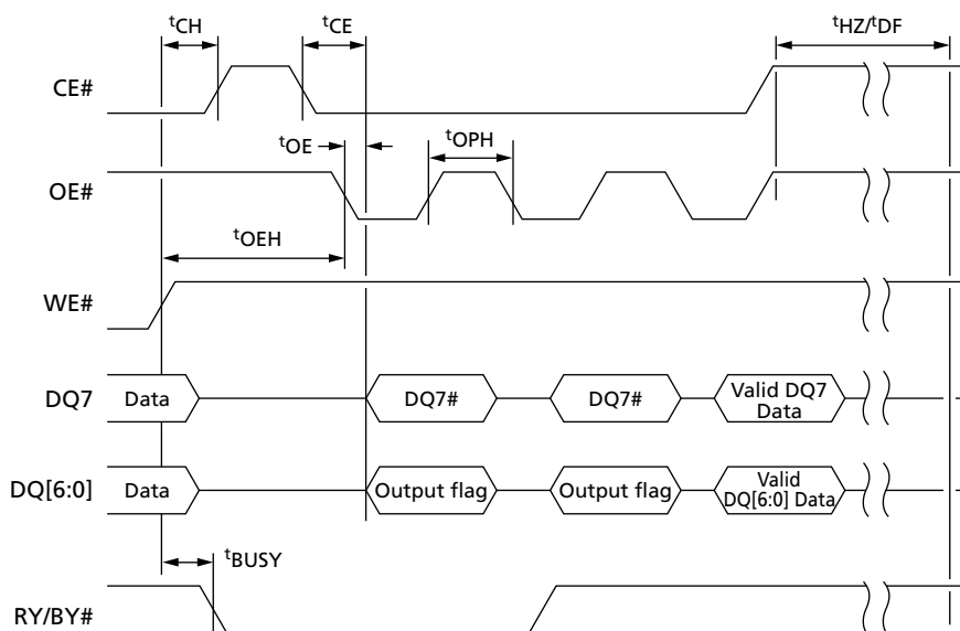
Figure 26: Data Polling AC Timing
