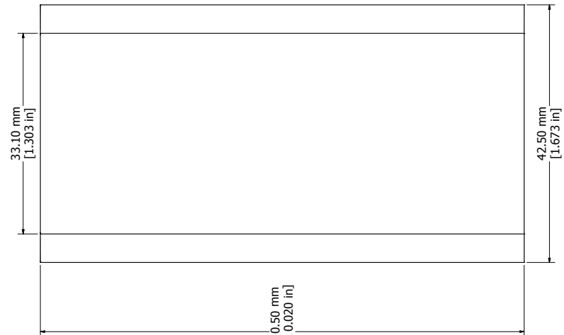
EXTRUSION PROFILE
