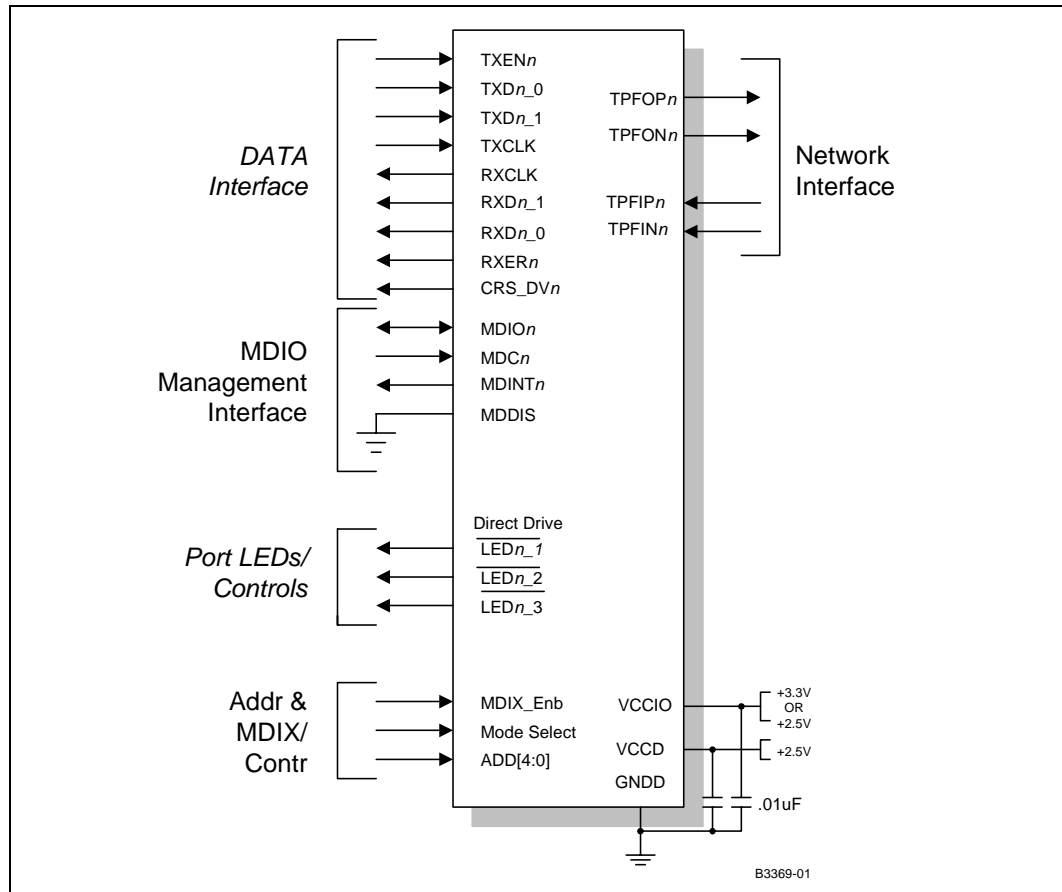
Figure 7 Interface Signals
