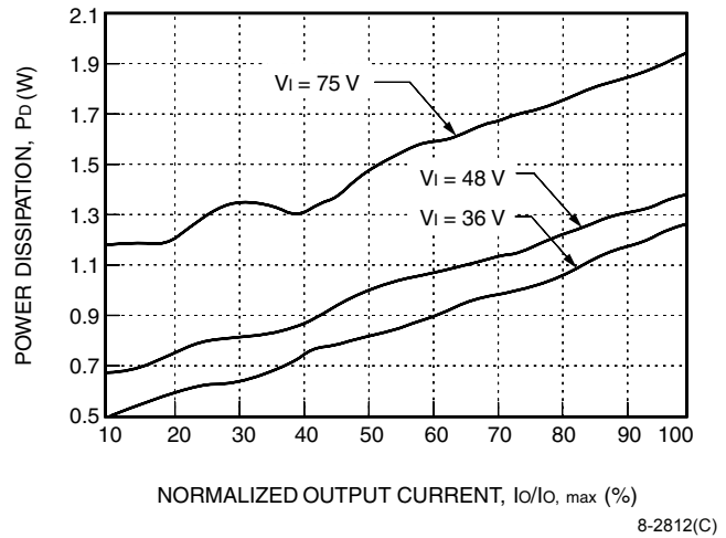
Figure 29. LW005C Power Dissipation vs. Output Current
