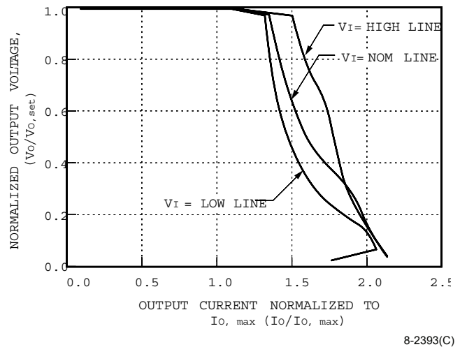
Figure 4. Lx005x Normalized Output Current vs. Normalized Output Voltage at T_c = 25\text{ °C}
