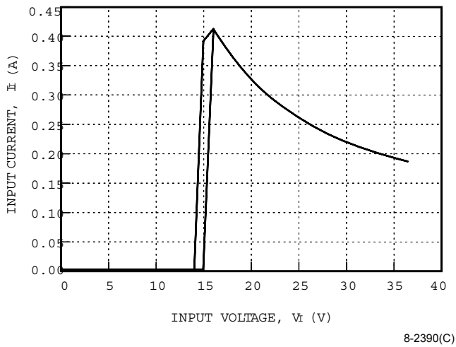
Figure 1. LC005x Input Current vs. Input Voltage at I_o = I_{o,max} and T_c = 25\text{ °C}
