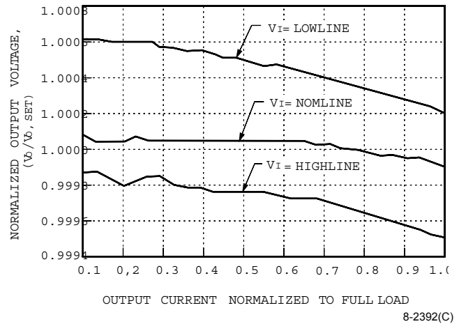
Figure 3. LW005x Load Regulation, Normalized Output Voltage vs. Normalized Output Current at T_c = 25\text{ °C}
