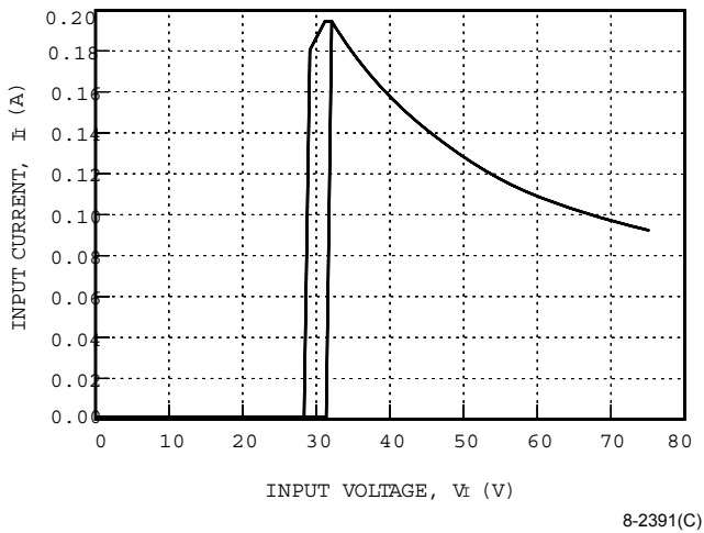
Figure 2. LW005x Input Current vs. Input Voltage at I_o = I_{o,max} and T_c = 25\text{ °C}
