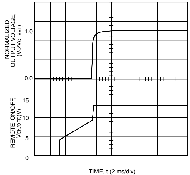
Figure 15. Typical Output Voltage Start-Up when Signal Is Applied to Remote On/Off; I_o = I_{o, max} V_i = \text{Nominal Line} at T_c = 25^\circ C
