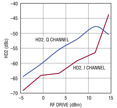
HD2 at 150MHz IF vs RF Drive
