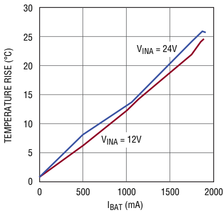
Temperature Rise vs I BAT , 4.1V BAT
