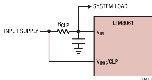
Figure 3. R_{CLP} Sets the Input Supply Current Limit
