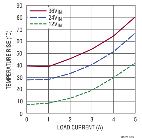
Temperature Rise vs Load Current 8V_{OUT}
