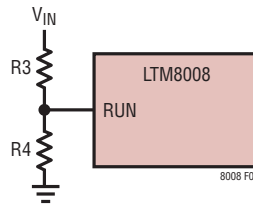
Figure 1. The LTM8008 Turn-On and Turn-Off Thresholds Are Set by a Simple Resistor Network
