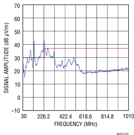
Figure 33. Radiated Emissions Scan of LTM4676 Producing 1V OUT at 26A, from 12V IN . DC1811A Hardware with Outputs Paralleled. 1\Omega (1/4W rated) Snubber Resistors Applied from \text{SNUB}_n to GND. f_{\text{SW}} = 350\text{kHz} . Measured in a 10m Chamber. Peak Detect Method
