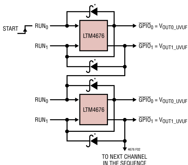
Voltage Based Sequencing by Cascading \overline{\text{GPIO}}_n Pins Into \text{RUN}_n Pins (MFR_GPIO_PROPAGATE = XXX1X00XX00XXXXX h and MFR_GPIO_RESPONSE = 0x00)
