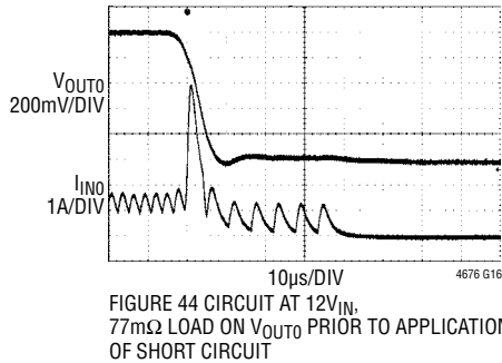
Single Phase Single Output Short-Circuit Protection at Full Load
