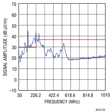
Figure 32. Radiated Emissions Scan of LTM4676 Producing 1V OUT at 26A, from 12V IN . DC1811A Hardware with Outputs Paralleled. No Snubbers Applied. f_{\text{SW}} = 350\text{kHz} . Measured in a 10m Chamber. Peak Detect Method
