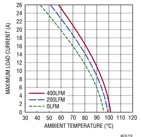
Figure 19. 24V to 1V Derating Curve, with Heat Sink
